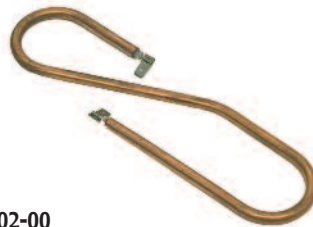
890-02-00 Heat Element 110 V, 900 W. Pkg: 1 ea. For Taylor 4" irons, Roberts 182 style & Orcon std. width irons.
